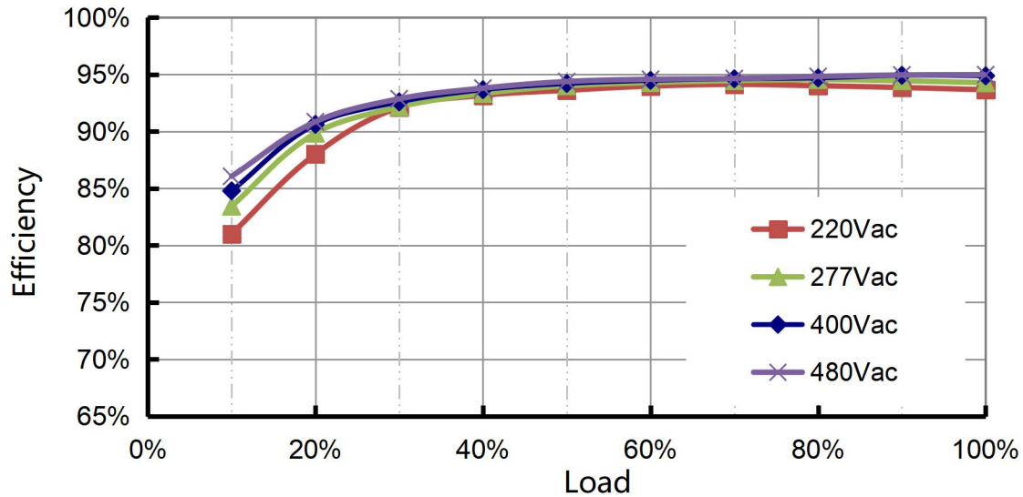
Efficiency vs. Load (C16A)
